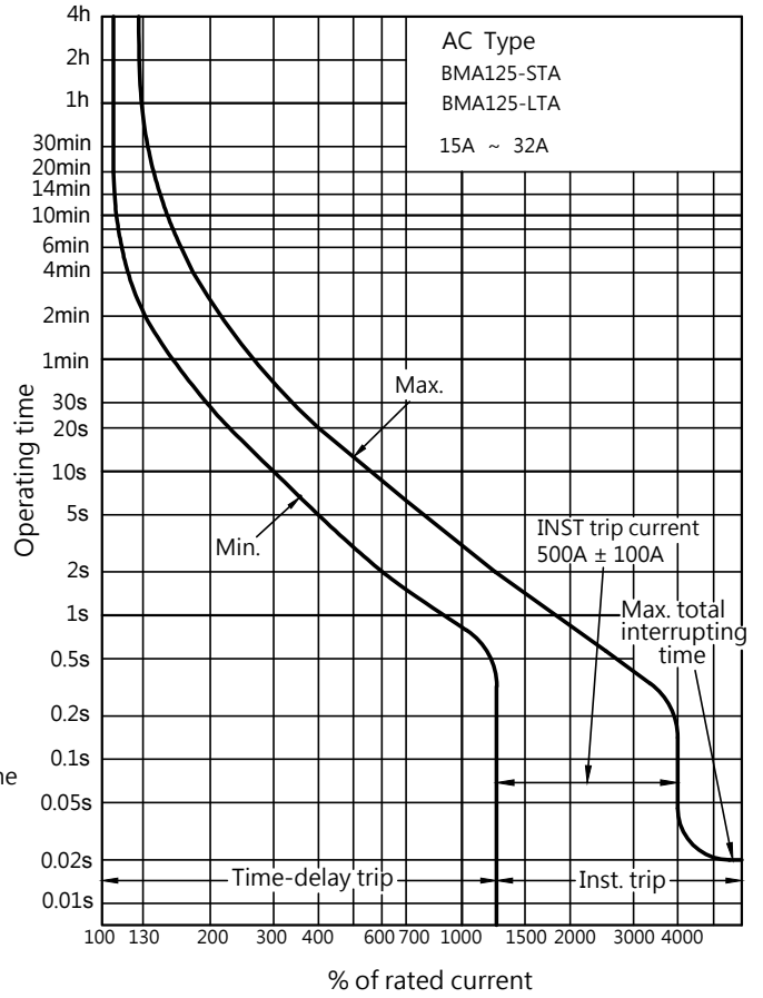
Operating Characteristics
