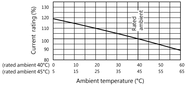
Compensation Curve
