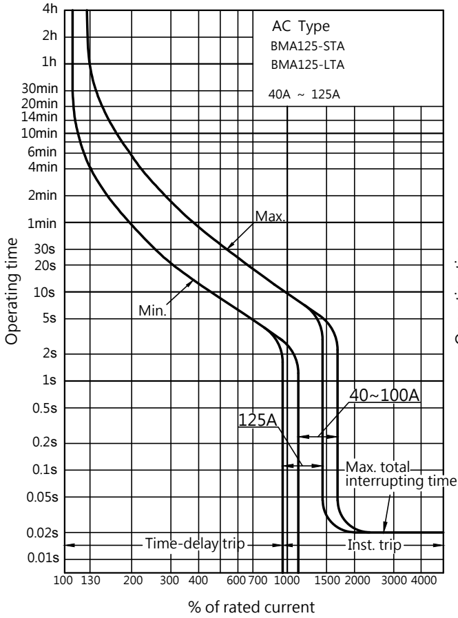
Operating Characteristics
