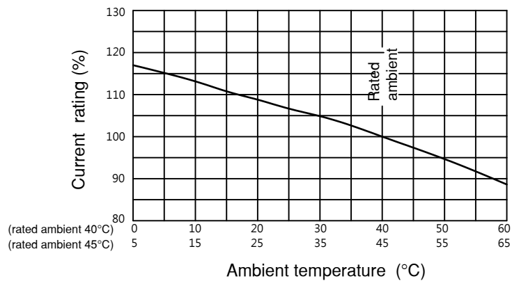
Compensation Curve
