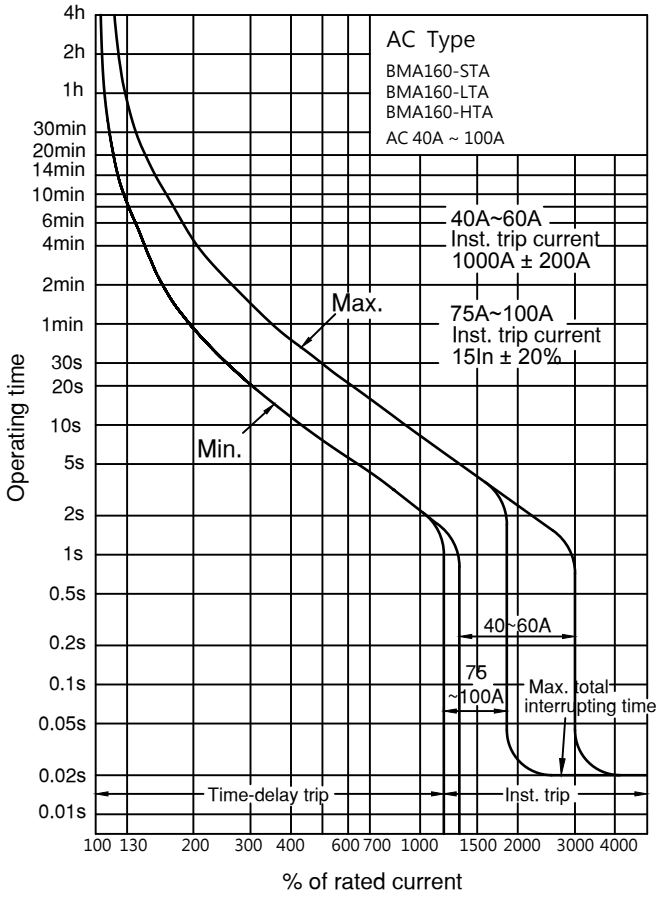
Operating Characteristics
